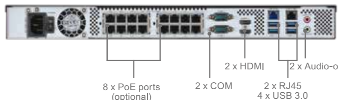
Rear I/O
