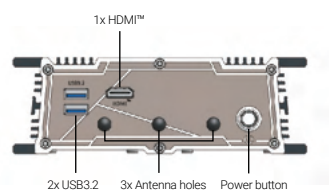
POC-766AWP-DEV Development version
